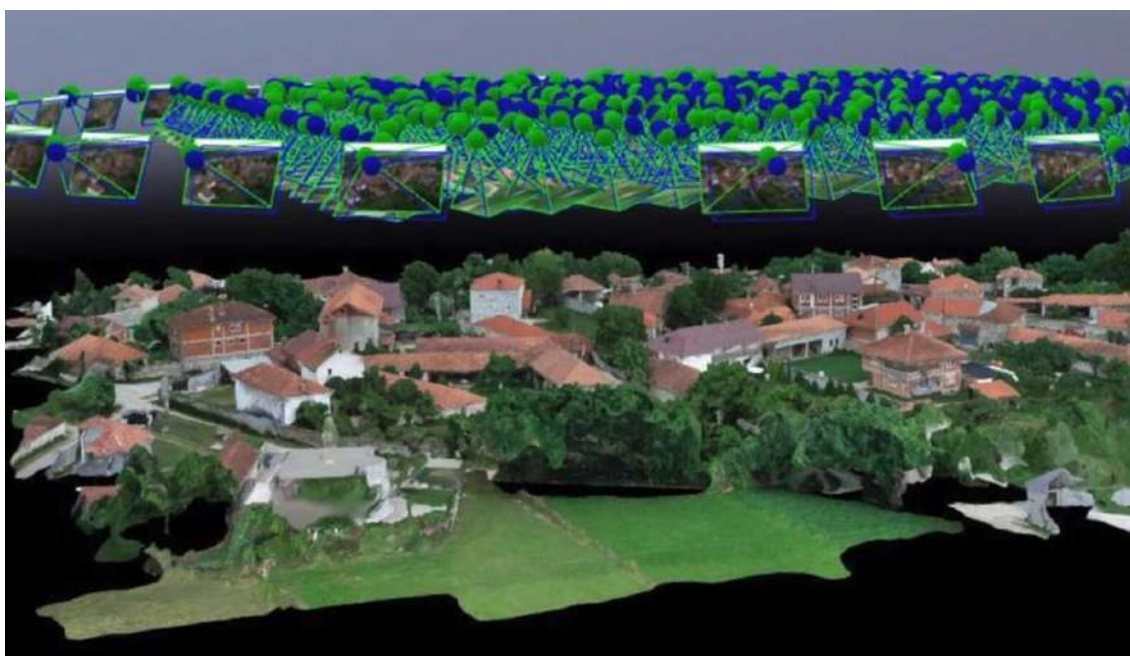
Figure 4: Recreating the Model in Pix4Dmapper.
