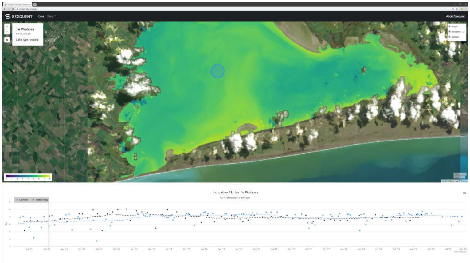
Figure 3: Indicative TLI Water Quality Information for Te Waihora in the Canterbury Region of the South Island of New Zealand Shown In SLIMS.
